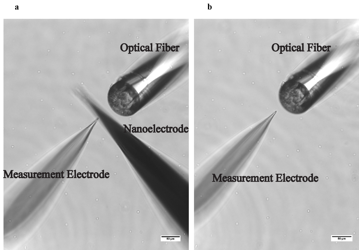
Figure 2.5: Digital micrographs were taken during the plasmonic temperature measurement at the surface of the nano-electrode. (a) The digital micrograph of the plasmonic temperature measurement experiment showing the nano-electrode, a patch pipette filled with extracellular solution, known as the measurement electrode, placed near the nano-electrode surface; and a 50 \mu\text{m} inside diameter optical fiber used to focus a 532 nm green laser on the surface of the nano-electrode (b) The control experiment showing the measurement electrode and a 50 \mu\text{m} inside diameter optical fiber (no nano-electrode).
