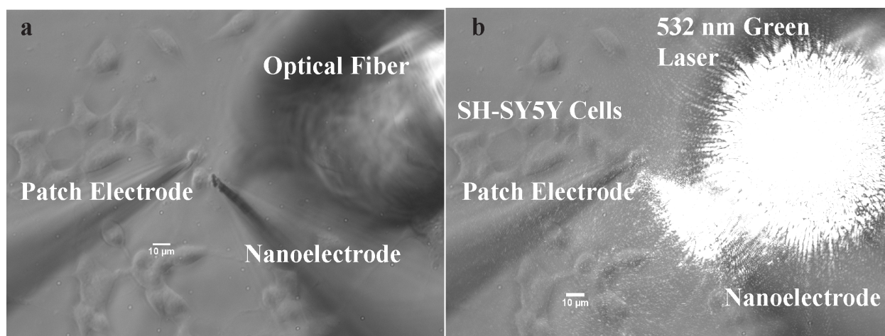
Figure 2.6: Digital micrographs showing the plasmonic set up in which our nanoelectrode was placed just next to an SH-SY5Y cell, and a recording microelectrode was used to patch the cell in whole-cell configuration. An optical fiber having an inside diameter of 50 \mu\text{m} was used to focus laser on the tip of the nanoelectrode (a) when laser was off and (b) when laser was on.
